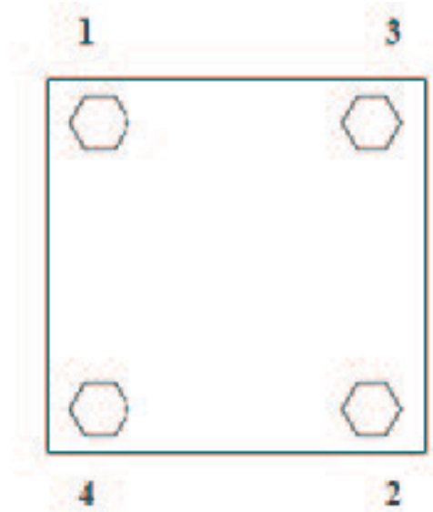
Figure 1 Tie Rod Nut Torquing Sequence
