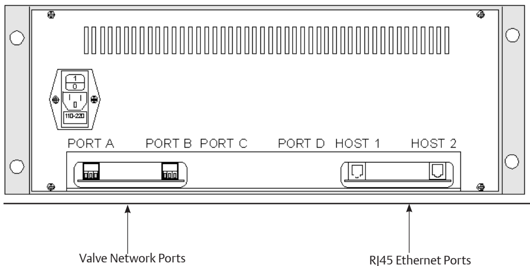
Figure 8 Rear Panel View
