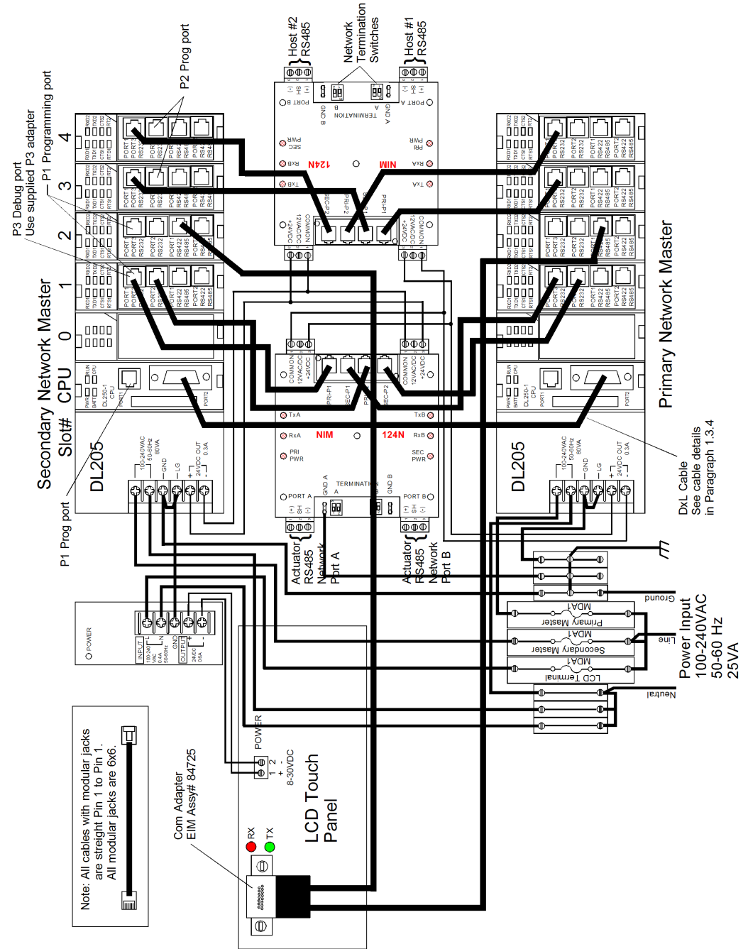
Figure 2 M250 NEMA TP Internal Wiring
