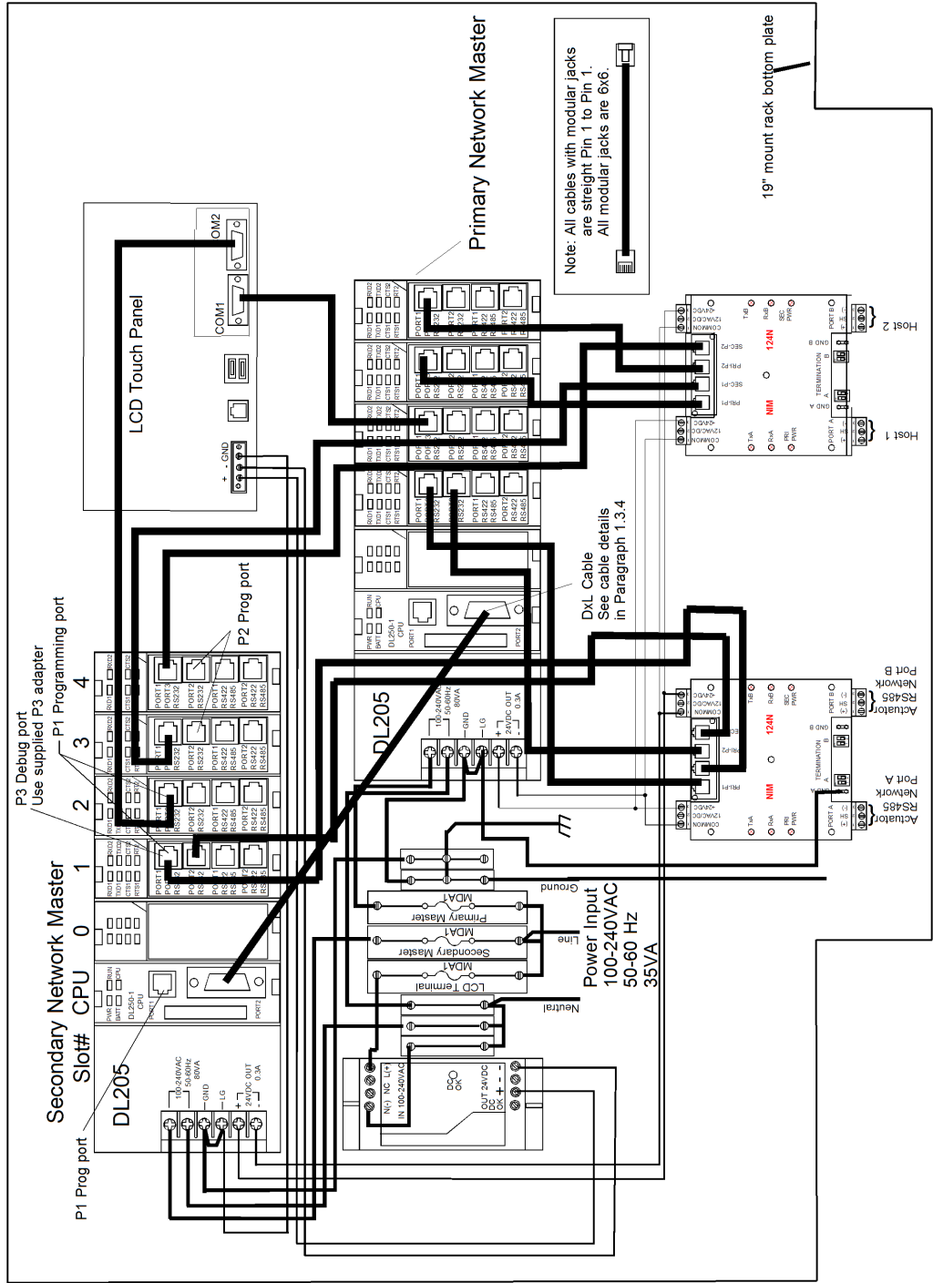
Figure 3 M250 Rack Mount TP Internal Wiring
