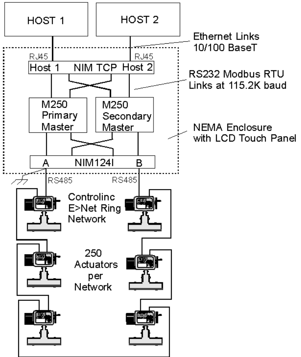
Figure 1 DCS System Diagram
