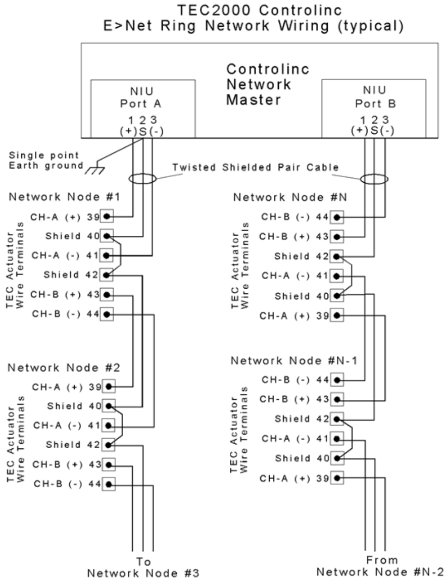
Figure 10 TEC2000 Controlinc E> Net Ring Network Wiring (Typical)
