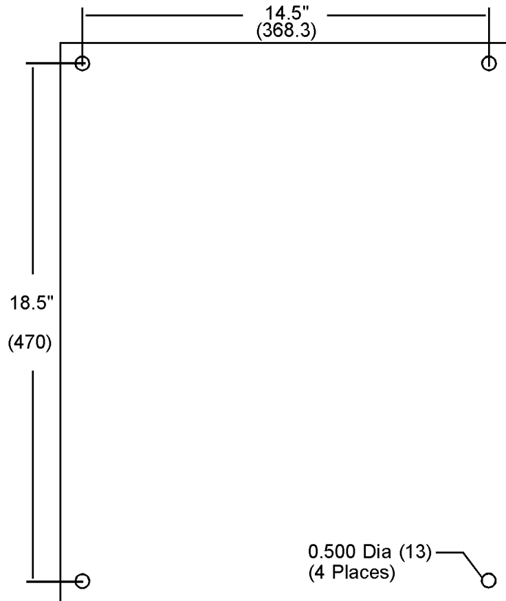
Figure 6 NEMA Box Mounting
