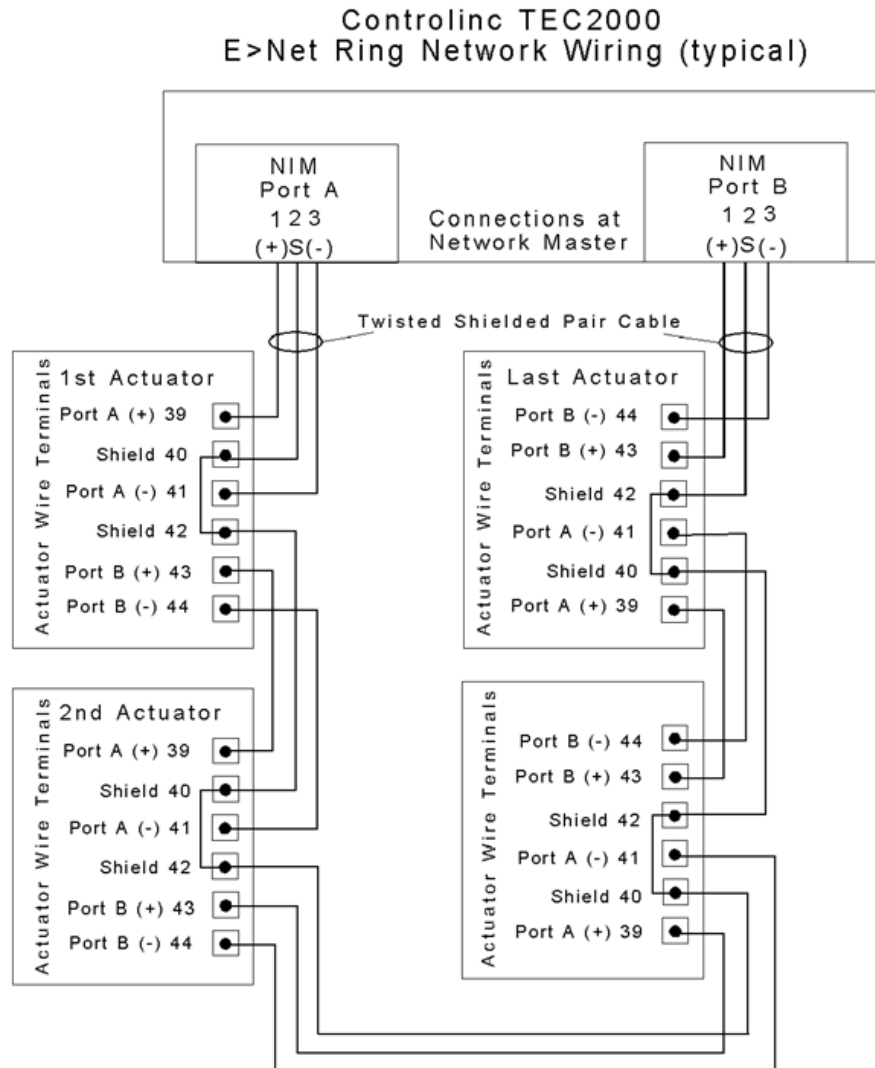
Figure 9 Controlinc TEC2000 E > Net Ring Network Wiring (Typical)
