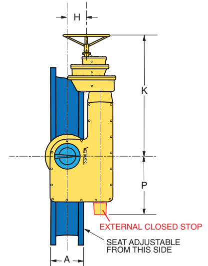
96" - 120" Actuator Orientation
