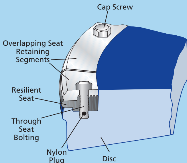
Figure 1. Tri-Loc™ Seat Retention System
